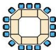
Delta 45 degree with Rectangles Overall Dimensions 3800W x 3800D
