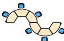
Curved Trapezoidal Overall Dimensions 5600W x 3200D
